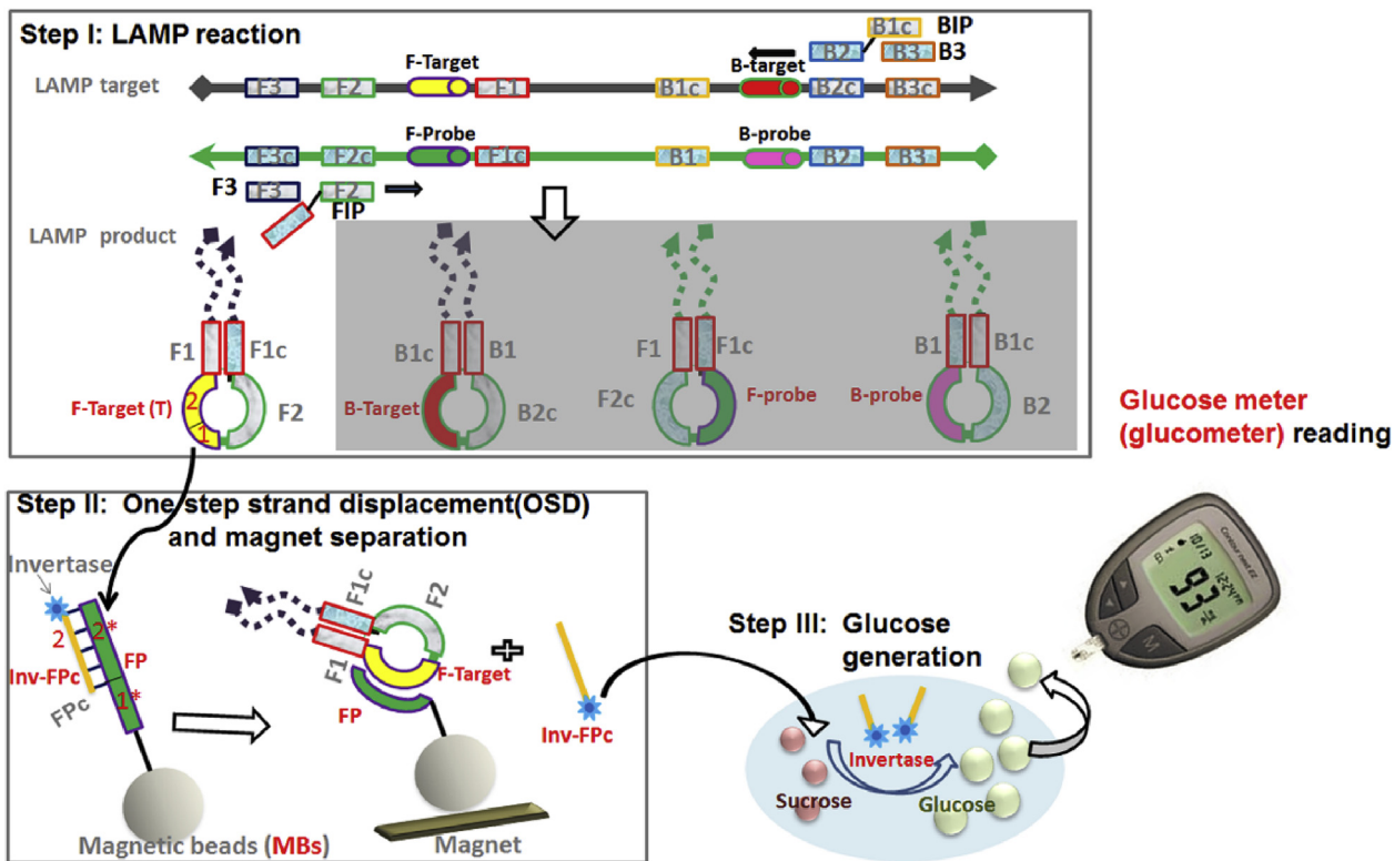
Fig. 2. Scheme for adapting isothermal amplification to a glucometer. The figure was reproduced with permission from Ref. [32].
