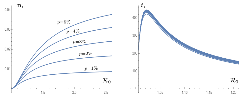
FIGURE 7. Left: size of the epidemic peak as a function of \mathcal{R}_0 . Right: date of the epidemic peak as a function of \mathcal{R}_0 . Plots correspond to p = 0.01, 0.02, \dots, 0.05 .
