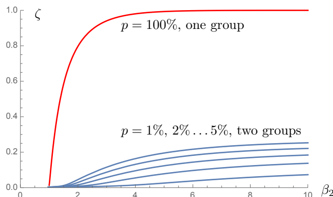
FIGURE 2. Epidemic size \zeta as a function of \beta_2 for p = 0.01, 0.02, \dots 0.05 (blue; n = 2 ) and p = 1 (red, n = 1 ). This red curve corresponds to an outbreak with a basic reproduction ratio \beta_2/\gamma . This is however not so instructive as the k = 2 group is a small proportion of the population, but with high transmission rate.
