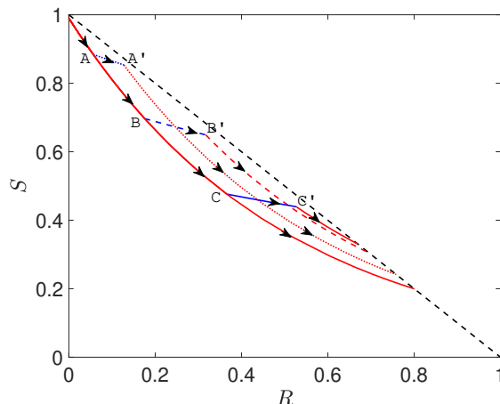
Figure 11: (S,R) phase portrait (arrows indicate growing time) based on an SIR model in a single population with \beta = 2 , \gamma = 1 (giving \mathcal{R}_0 = 2 ) and initial condition I(0) = 0.01 . The plot shows a trajectory with no control (continuous red line) as well as three other trajectories where \beta = 0.5 for a time period of length D = 2 but with the intervention setting in only once I + R goes past 0.1 (partially dotted line), 0.3 (partially dashed line) and 0.5 (continuous broken line), respectively. Control for the three different scenarios sets in at the points denoted by A, B and C and control ends at A', B' and C', respectively.
