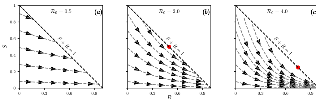
Figure 10: We plot S(t) versus R(t) for \mathcal{R}_0 = 0.5 (a), 2 (b), and 4 (c). For given S(t) and R(t) , the proportion infected is I(t) = 1 - S(t) - R(t) , which equals the vertical or horizontal distance from the point (R(t), S(t)) to the line S + R = 1 . The curves and arrows show how a solution to System (1) evolves in time. At points S > 1/\mathcal{R}_0 (which occurs only for \mathcal{R}_0 > 1 ) orbits move farther from the diagonal, representing an increase in I . Note that the velocity an orbit is traversed varies depending on location, and goes to zero close to S + R = 1 . Red dots in panel (b)-(c) indicate the point (S = \frac{1}{\mathcal{R}_0}, I = 0, R = 1 - S) .
