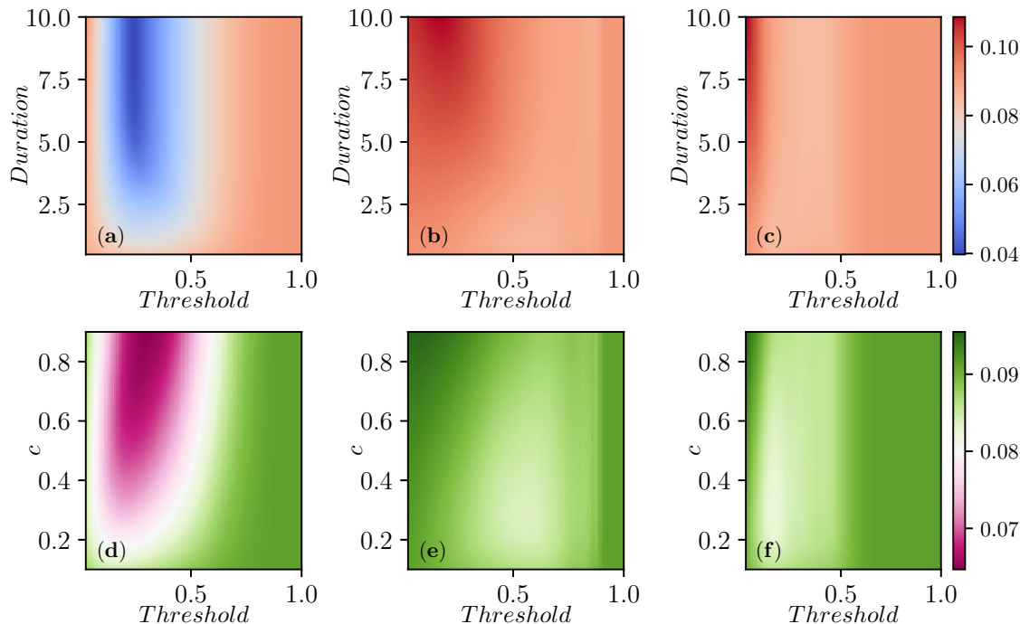
Figure 7: Contour plots of the peak prevalence I_{peak} = \max_t \left( \frac{1}{9} \sum_i I_i(t) \right) , averaged across 100 simulated populations each with 9 subcommunities. Control strategies and setup the same as in Figure 5.
