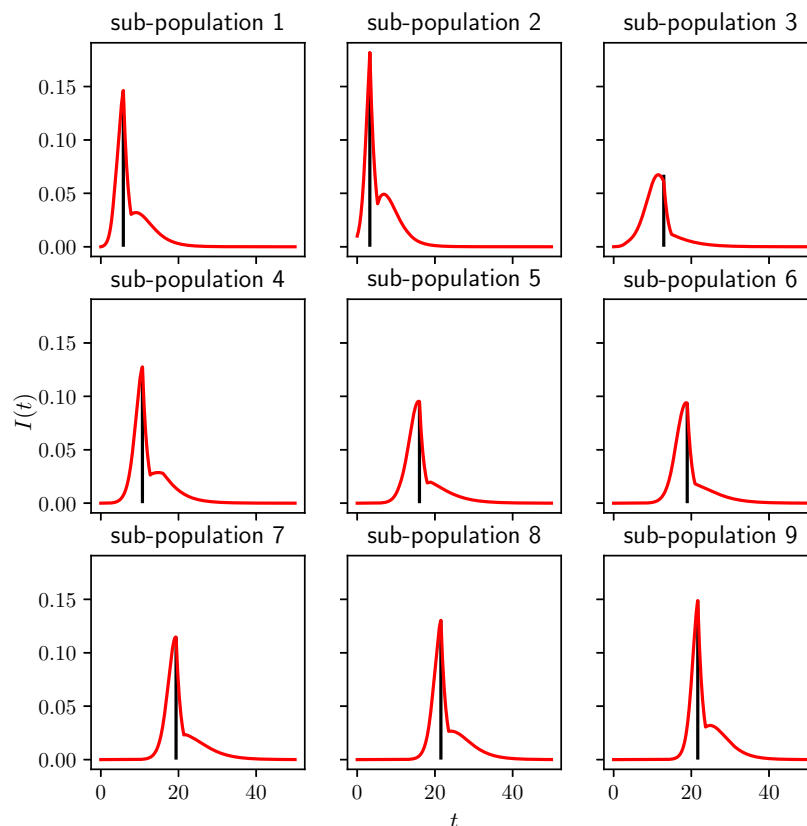
Figure 6: Illustration of best control strategy (i.e. smallest attack rate) (controlling subcommunities individually but using the same threshold for each) when efficacy and duration of control are fixed at c = 0.8 and D = 2 , respectively. It turns out that the optimal threshold is close to (0.4). This combination represents the point (0.4, 2) in Fig 5 panel (a), or equivalently the point (0.4, 0.8) in panel (d). With this strategy, we find that R(\infty) goes from R(\infty) = 0.75 to R(\infty) = 0.63 . If we increase control duration from 2 to 10 we would achieve a further reduction to R(\infty) = 0.44 . The vertical black lines show the onset of control.
