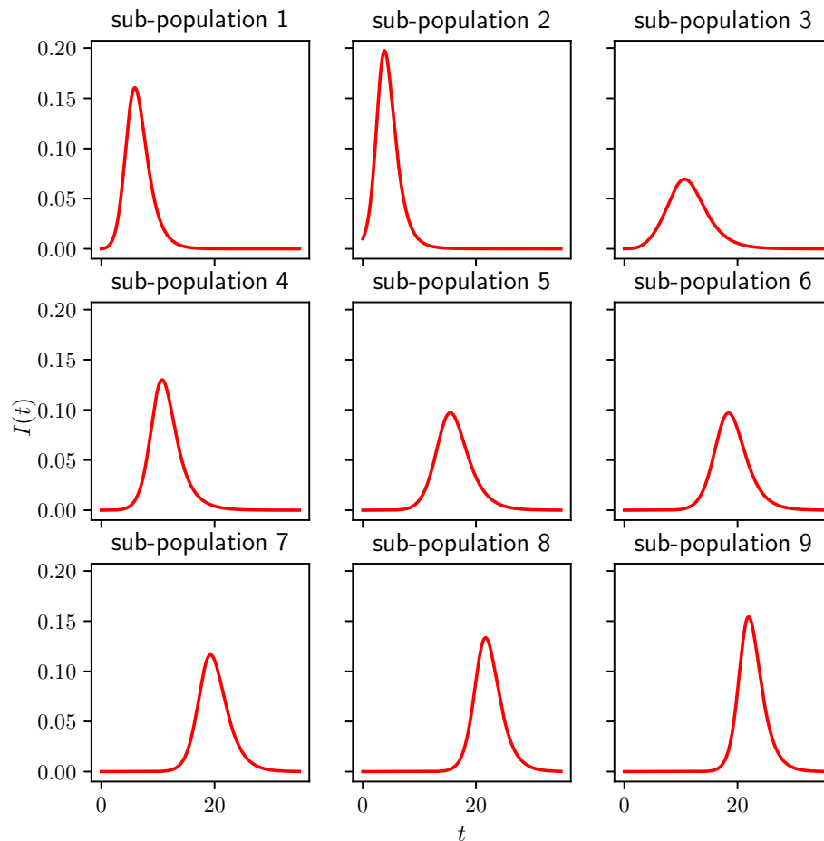
Figure 4: Example of an epidemic spreading across 9 subcommunities with different contact rates (see the Appendix A.2 for the precise mixing matrix B ). The epidemic starts from subcommunity 2 and it is run for T = 35 units of time. \gamma = 1 for all subcommunities. With no control the attack rate or final epidemic size is 0.744.
