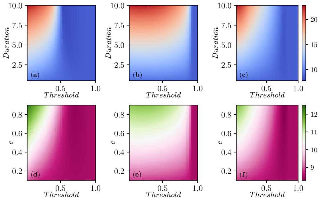
Figure 9: Contour plots of the global mean infection time, defined as T = -\frac{1}{R(\infty)} \int_0^\infty t \sum_i \frac{dS_i}{dt} dt , averaged over 100 simulations. In terms of control strategies and parameter values the same setup as in figures 7 and 5 are used.
