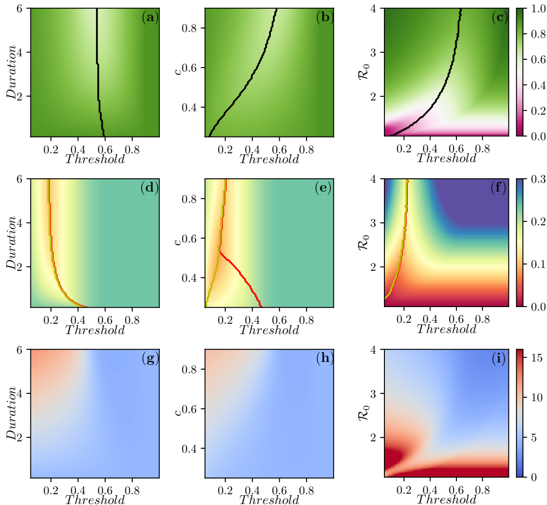
Figure 3: Contour plots for R(\infty) (top), I_{\max} (middle) and the mean time of infection \bar{t} (bottom) as a function of parameters for the well-mixed population. We explore different threshold values of I + R for the intervention to start, from a minimum of 0.05 to a max of 0.9. The first column investigates the impact of duration from D = 0.1 to D = 6 , holding \beta = 2.5 and c = 0.8 . On the second column, intervention duration is D = 4 and c ranges from 0.2 to 0.9. Finally, on the third column, c = 0.8 and D = 4 , and the values of \beta = \mathcal{R}_0 vary from 1 to 4. In all cases \gamma = 1 . In the first row, the black curve denotes the threshold for which \mathcal{R}_e = 1 when the intervention completes. In the three regions defined by the two lines in the panels of the second row, the peak prevalence is observed after the intervention has ended (from left to yellow curve), during intervention (area between the curves), or before intervention (from red curve to the end of the figure). Where the two curves align, the prevalence decays as soon as the intervention is implemented and then recovers to the pre-intervention peak.
