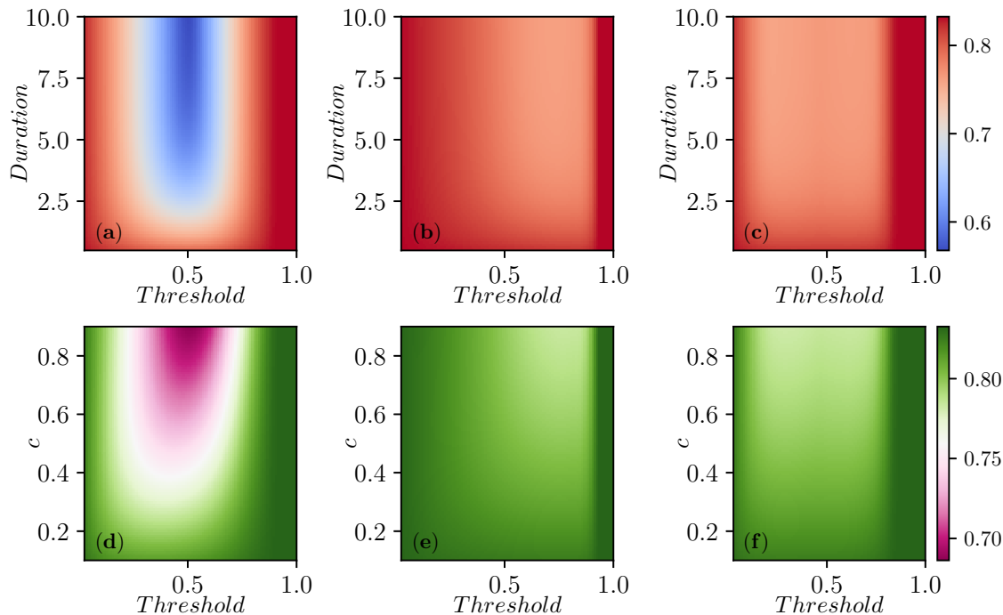
Figure 5: Contour plots showing the average attack rate (final epidemic size) over 100 simulated populations for each set of parameter values. In the first row c is fixed and the duration of control varies on the vertical axis, while in the second row duration is fixed and c varies. Each column corresponds to one of the three strategies: (a,d) intervention in each subcommunity, (b,e) global intervention when the first subcommunity breaches the threshold, and (c,f) global intervention at global threshold for a population consisting of 9 subcommunities. In each plot, the x -axis shows the values that the threshold for intervention can take (from a minimum of 0.05 to a maximum of 0.8). In the first row c = 0.8 is constant, while the duration of control varies from a minimum of T = 1 to a maximum of T = 10 . On the second row instead, the duration of control is kept fixed at T = 2 , and the values of c varies from c = 0.1 to c = 0.9 . The recovery rate is \gamma = 1 for all subcommunities. In all cases, if the threshold is set too large the intervention is never implemented. The two synchronized interventions can be approximately mapped to one another by noting the largest I_i + R_i at the time the global I + R reaches a given threshold. The subcommunity threshold gives more resolution at small values while the global threshold gives more resolution at large values.
