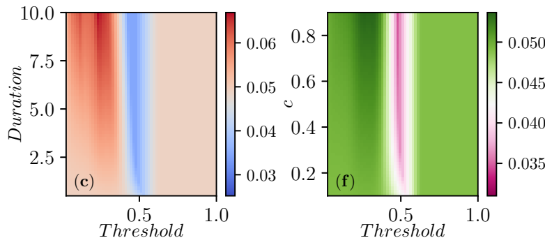
Figure 8: Contour plots of the peak prevalence, I_{peak} , that is the maximum value achieved by I(t) = \frac{1}{N} \sum_i I_i(t) during the time-course of the epidemic. Control strategies and setup the same as in Figure 5.
