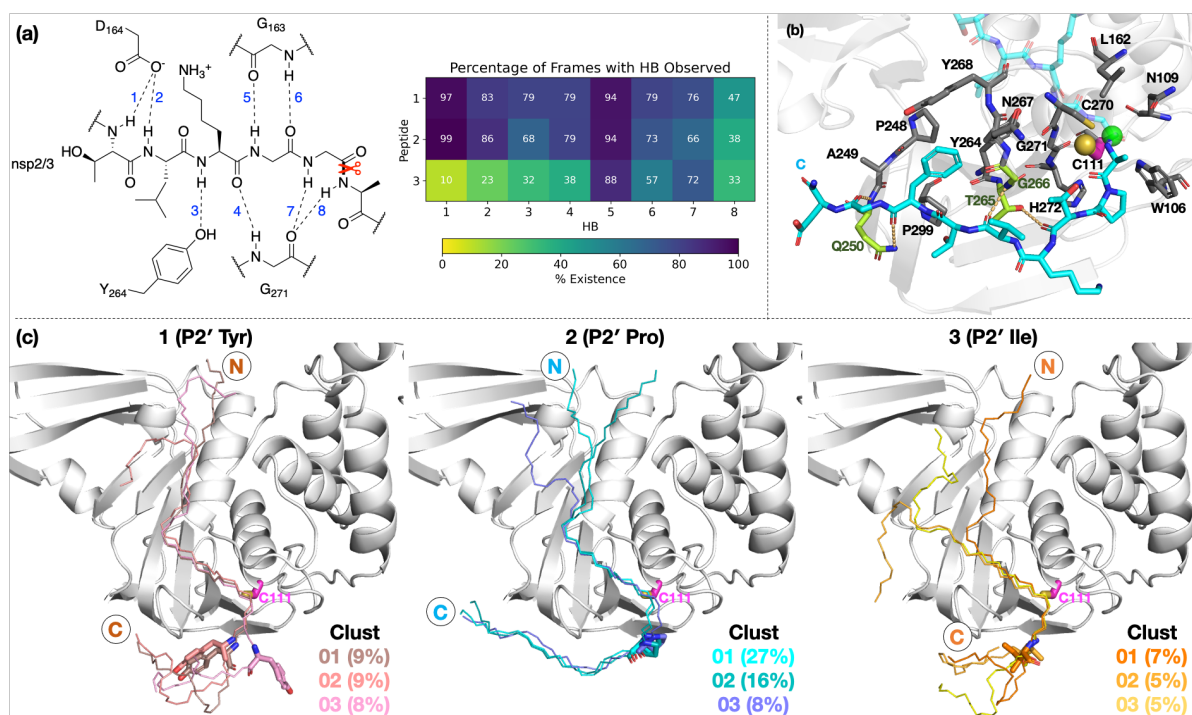
Figure 3: Interactions of PL pro with the oligopeptides 1, 2, and 3. (a) Conserved HBs (occurrence \geq 25\% for at least two peptides) in the P5-P1' region, observed in 3 \times 200 ns MD. (b) Representative structure of N-state PL pro complexed with 2 (cyan; P1 scissile amide carbonyl carbon as a green sphere) from cluster analysis (peptide backbone RMSD cut-off of 3 Å) highlighting interactions in the P' region. PL pro residues involved in HBs are shown in lime. Residues within 4 Å of P' residues are in grey, except for Cys111 which is in magenta (its sulfur as a yellow sphere). (c) View of representative structures of the three most populated clusters, from the combined 3 \times 200 ns MD of each of the three PL pro -peptide (N state) complexes. The peptide backbone is shown as thin sticks and the P2' residue as thick sticks.
