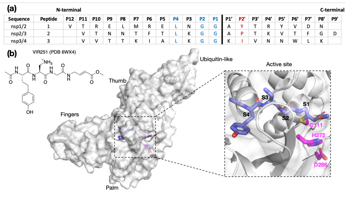
Figure 1: (a) Sequences of the reported oligopeptides used in SARS-CoV-2 PL pro mass spectrometry-based assays. 22 The consensus LXGG sequence residues are in blue; the P2' residues are in red. (b) View from a reported PL pro structure (PDB 6WX4) 13 in complex with the covalently bound inhibitor VIR251 (carbon atoms in violet), which binds to the S1-S4 subsites; the catalytic triad residues are shown (carbon atoms in magenta). Non-carbon atoms are colored: N in blue; O in red; S in yellow; Zn in gray. Hydrogens are omitted for clarity.
