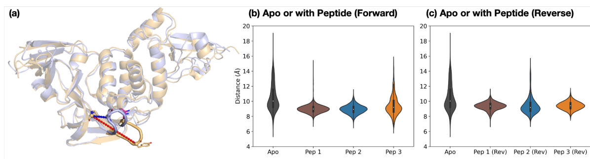
Figure 5: Dynamics of the Tyr268-containing loop PL pro BL2. (a) Views of MD-observed structures of apo PL pro when BL2 is closed (light blue) and open (light orange), which can be quantified by the Pro248–Tyr268 Ca–Ca distance (blue and red dotted lines respectively). The distribution of this distance over combined 3 \times 200 ns MD is plotted for PL pro in the apo state and (b) when complexed with the nsp peptides in the forward binding mode, and (c) when complexed with the nsp peptides in the reverse binding mode.
