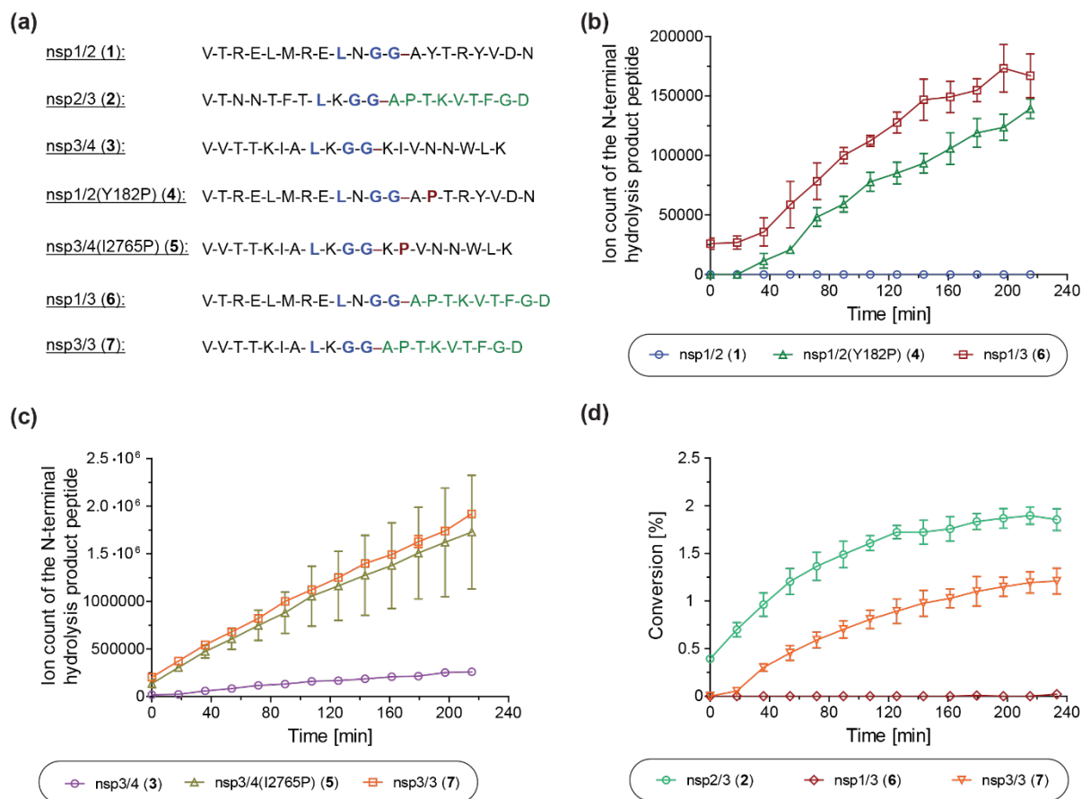
Figure 6. A proline at the substrate P2' position enhances PL PRO catalysis. (a) Sequences of the employed SARS-CoV-2 polyprotein-derived oligopeptides used; (b) ion counts of the N-terminal hydrolysis product peptides of wt nsp1/2 (1; blue circles), nsp1/2(Y182P) (4; green triangles), and nsp1/3 (6; red boxes) incubated with SARS-CoV-2 PL PRO ; (c) ion counts of the N-terminal hydrolysis product peptides of wt nsp3/4 (3; lavender circles), nsp3/4(I2765P) (5; ochre triangles), and nsp3/3 (7; orange boxes) incubated with SARS-CoV-2 PL PRO ; (d) conversion of the PL PRO -catalyzed hydrolysis of wt nsp2/3 (2; light green circles), nsp1/3 (6; red diamonds), and nsp3/3 (7; orange inverse triangles), determined using the reported N-terminal acetylated C-terminal hydrolysis product peptide of 2 22 as an internal standard (0.2 \mu M). Reactions were performed using peptide (2.0 \mu M) and SARS-CoV-2 PL PRO (0.2 \mu M) in buffer (50 mM Tris, pH 8.0, 20 °C) and analyzed using SPE-MS under reported conditions. 22 Results are means of three independent runs ( n = 3 ; mean \pm standard deviation, SD).
