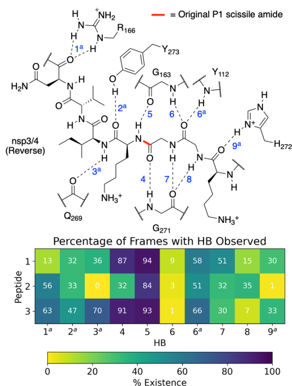
Figure 4: Possibility of reverse binding conformations for the oligopeptides 1, 2, and 3. Occurrence of conserved HBs during 3 \times 200 ns MD of PL pro complexed with the three nsp oligopeptides 1, 2, and 3 in the reverse binding conformations. The HBs are numbered according to the equivalent peptide position in Figure 3a , with additional HBs carrying the “a” superscript.
