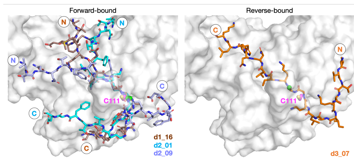
Figure 2: Predicted bound conformations of linear oligopeptides in complex with PL pro . AutoDock CrankPep (ADCP) 36 -predicted peptide conformations when non-covalently bound with PL pro (white surface), with PL pro Cys111 residue (magenta sticks) and the peptide N- and C-terminals labeled. The P1 scissile amide carbonyl carbon is shown as a green sphere. The poses are denoted by “dX_YY”, where “X” is the peptide number 1 , 2 , or 3 for the nsp1/2, 2/3, or 3/4 cleavage sites respectively, and “YY” the ranking out of 100 docked poses.
