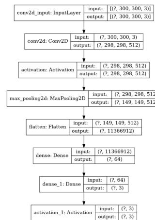
Fig. 3: Figure 5. Proposed CNN
