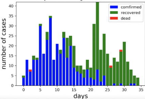
Daily cases in Shanghai after 2020-1-24
