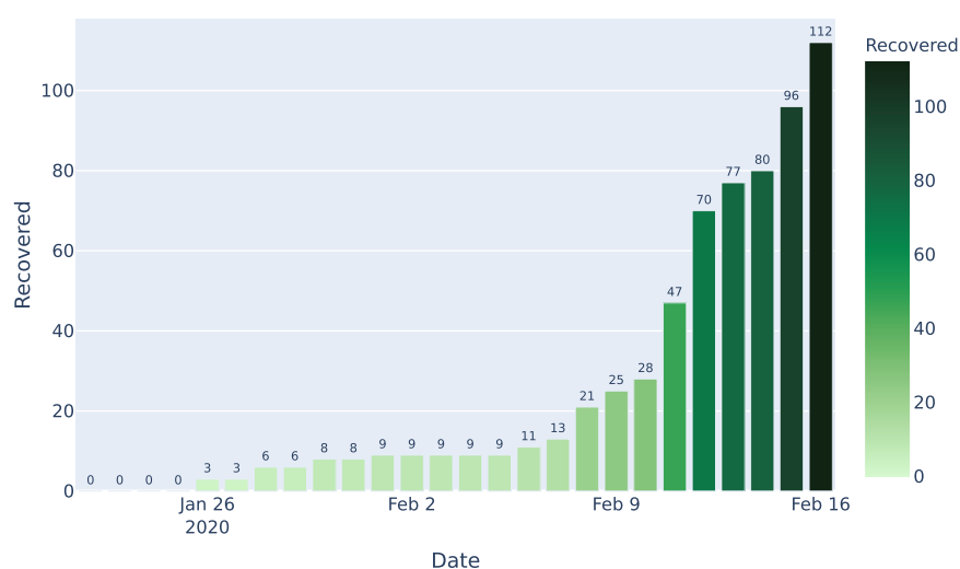
FIGURE 2 Exploratory data analysis of the number of recovered cases outside China with data visualization. It depicts that the rate of recovery outside China also increases regularly and till 16 February 2020, the number of recovered patients was 112 worldwide
