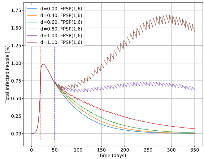
Fig. 15: Sensitivity analysis of the quantity I + D + A + R + T in the SIDARTHE model on increased infection rate (1 + d)\beta^+ during periodic working days. The FPSP-(1, 6) policy remains stable for d \leq 0.80 , corresponding to a 80% increase in infectious contacts during periodic working days due to compensatory and anticipatory population behavior.
