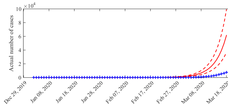
Figure 2: Distribution of the cumulated number of infected cases ( I(t) + R(t) ) across time. Solid line: average value obtained from the posterior distribution of the parameters. Dotted curves: 0.025 and 0.975 pointwise posterior quantiles. Blue crosses: data (cumulated values of \hat{\delta}_t ).
