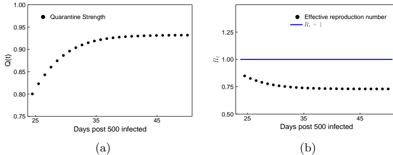
Figure 7: South Korea forecasting: (a) Quarantine strength Q(t) and (b) Effective reproduction number R_t , based on the neural network augmented SIR model.
