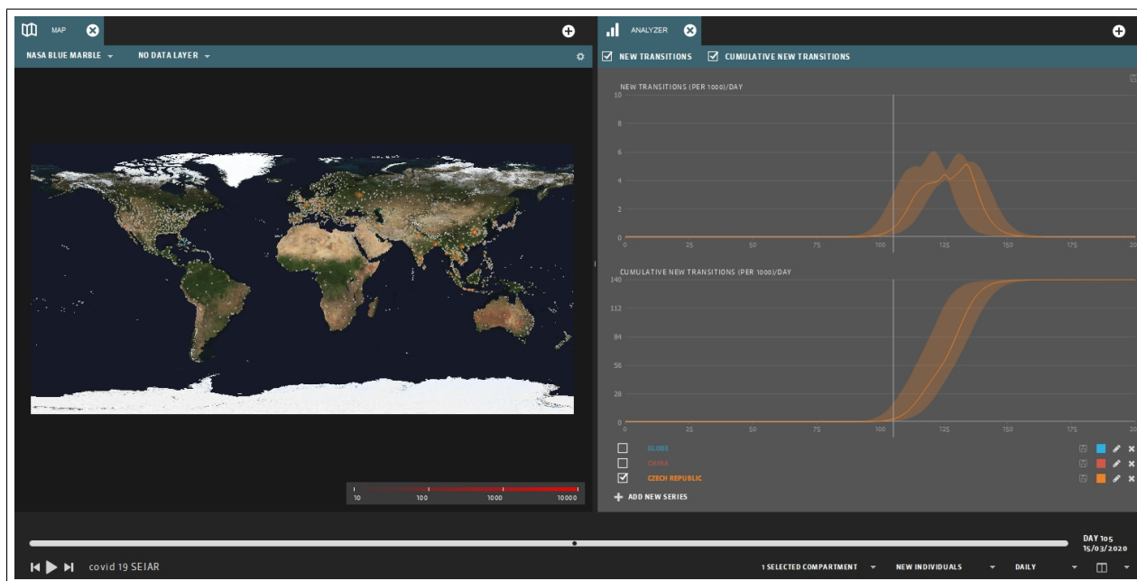
Figure 2: Global simulation of COVID-19 outbreak without European protective measures in GLEAMviz based on the model (1), (2), (3),(4) with parameters \beta = 1 , \gamma = 1/4 , \mu_1 = 1/3 , \mu_2 = 1/10 and p = 0.14 . Czech Republic – new transitions per 1000/day and cumulative transitions per 1000/day.
