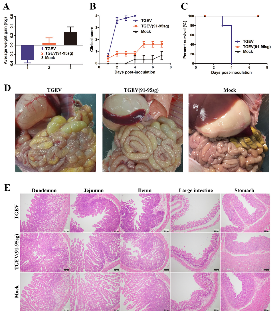
Figure 7. Pathogenicity analysis of TGEV and TGEV(91-95sg). A, piglets were inoculated with the viruses. The average weight gain of the piglets was recorded on the day of death or euthanasia as the final time point. In the TGEV group, one piglet died by the 3rd day, and the other piglets died by the 4th day. In the TGEV(91-95sg) and mock groups, the piglets were euthanized on the 8th day. Data are represented as mean \pm S.D., n = 3-5 . B, clinical mental state scores of the piglets in the different groups. The following criteria were used for evaluation: 0, normal; 1, mild lethargy (slow to move; head down); 2, moderate lethargy (stands but tends to lie down); 3, heavier lethargy (lies down; occasionally stands); and 4, severe lethargy (recumbent; moribund). Data are represented as mean \pm S.D., n = 3-5 . C, survival rates of the piglets in each group. Survival curves for the piglets infected with the recovered viruses in each group are shown. D, gross lesions in piglets inoculated with the recombinant viruses. The intestinal lesions were examined on the day of death or after euthanasia at the final time points. The necropsy images show transparent intestines observed in piglets inoculated with TGEV and TGEV(91-95sg) but not in mock-inoculated piglets. E, histopathological examination of the intestines from the recombinant TGEV-infected piglets. Different segments, including the duodenum, jejunum, ileum, large intestine, and stomach, were taken from each group and then processed for H&E staining. Representative images are shown. Original magnification \times 100 (scale bars 200 \mu m).
